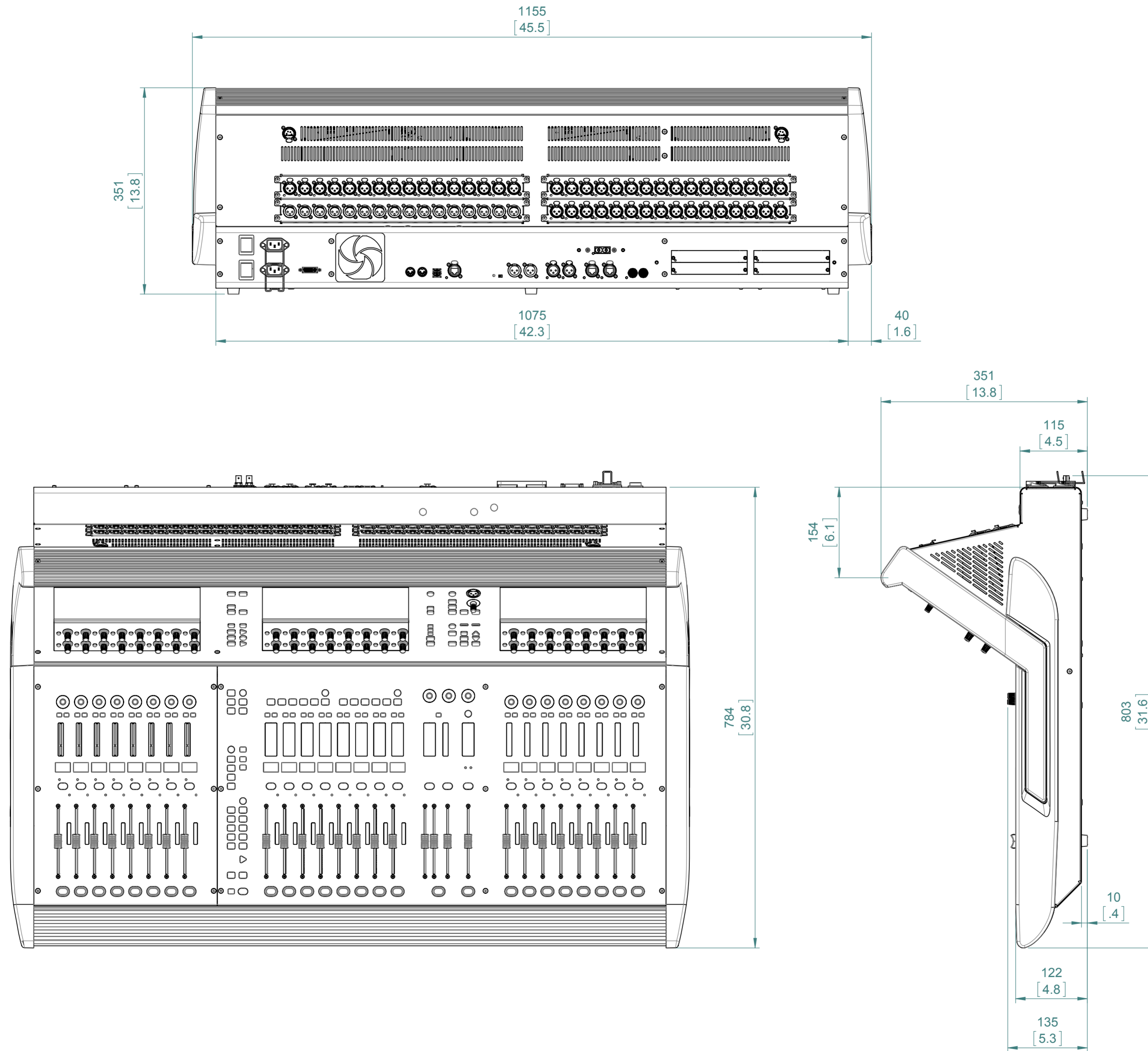
Vi2000 Outline Dimensions
